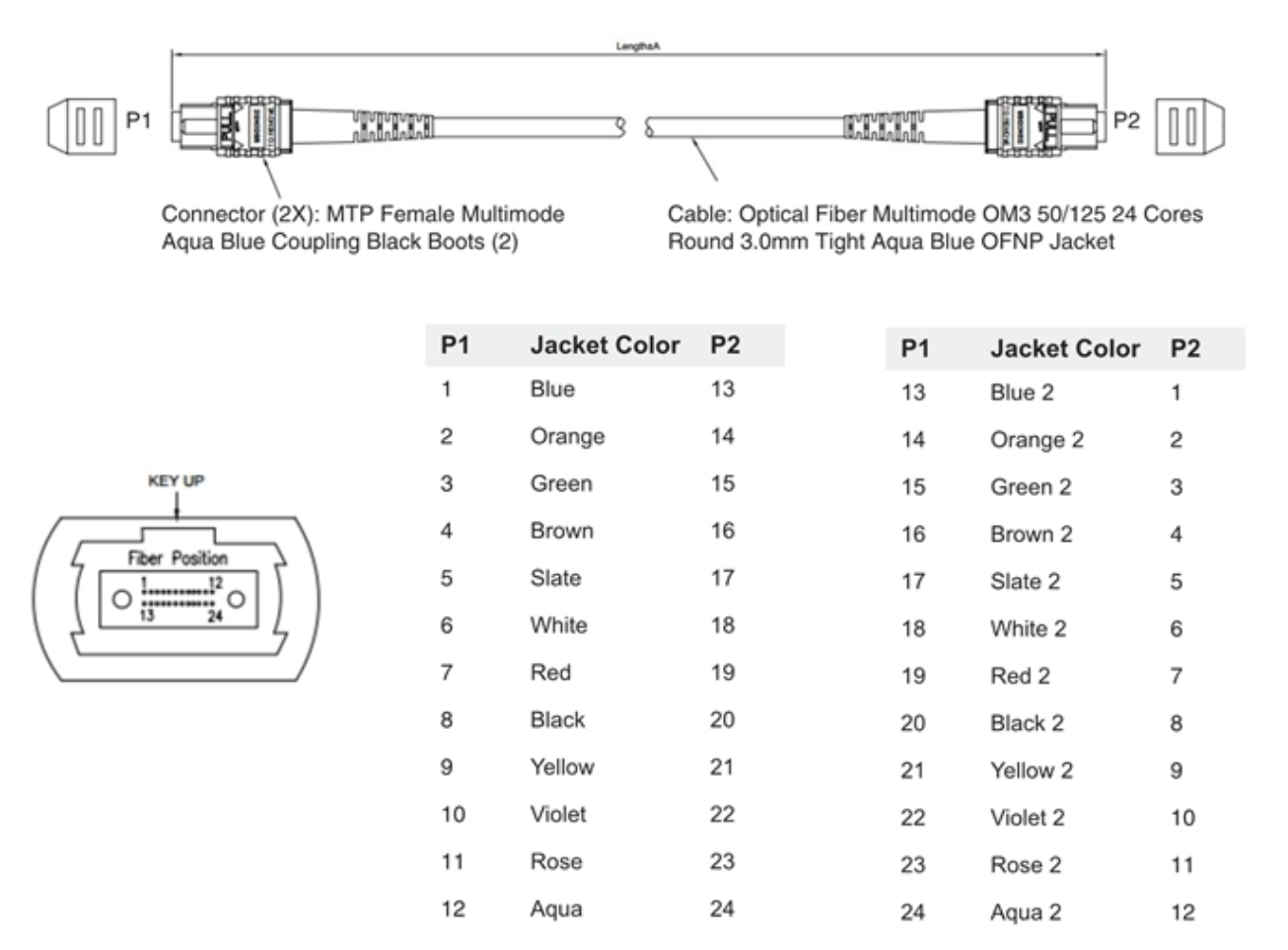
Figure 23 MPO/MTP 24 Position Fiber Cable
