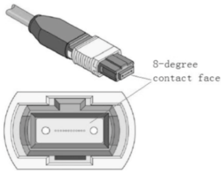
Figure 22 MTP/APC Cable
